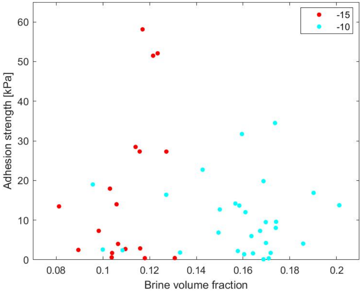
Figure 5: Adhesion strength of samples grown at -15 °C (red) and -10 °C (blue) plotted over the brine volume fraction of the samples.
