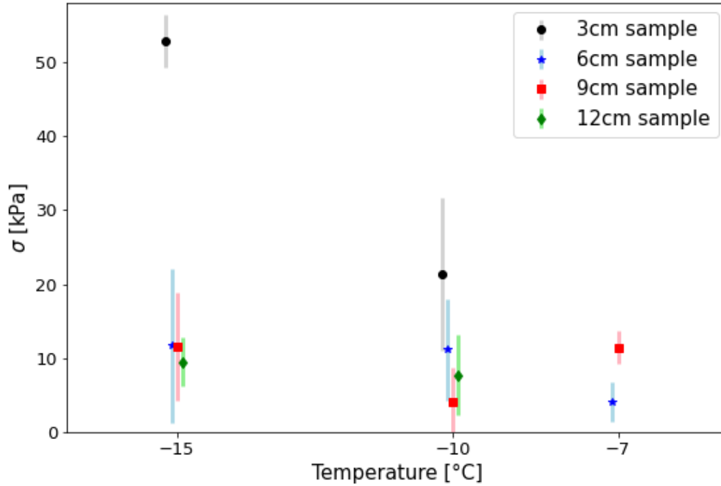
Figure 4: Overview of adhesion strengths of spray ice samples of different sizes.
