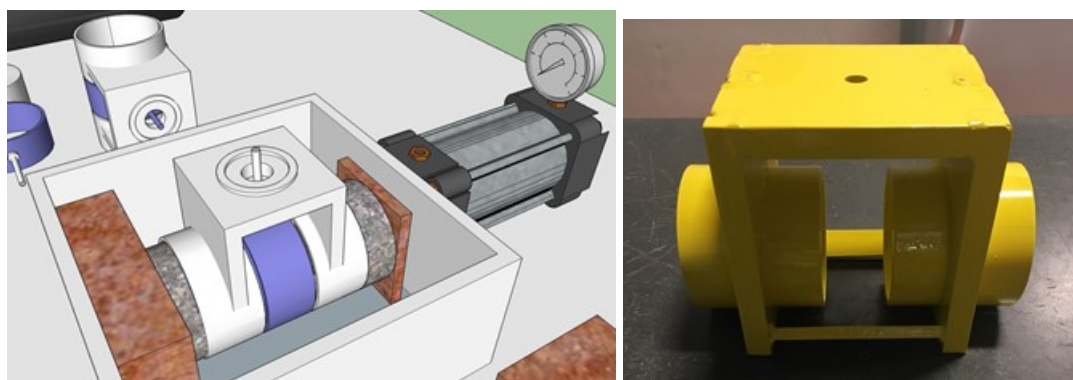
Figure 4 Double shear apparatus concept drawing (left) and as-built specimen holder (right).
