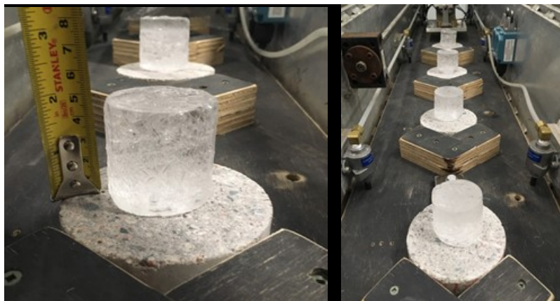
Figure 3 Ice samples ready for testing in direct shear.
