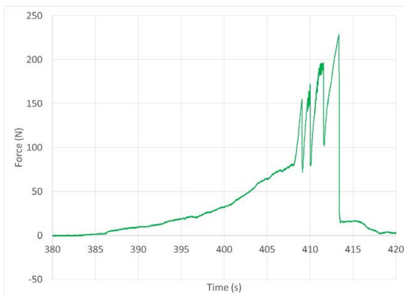
Figure 7 Measured loads for a sample, after 24 hours of loading with a 2.25 kg weight, at an air temperature of -11^{\circ}\text{C} . Failure is through the ice rather than the adhesive bond, per a series of cracking events, audible and visible in the video of the test, and observable in the load trace.
