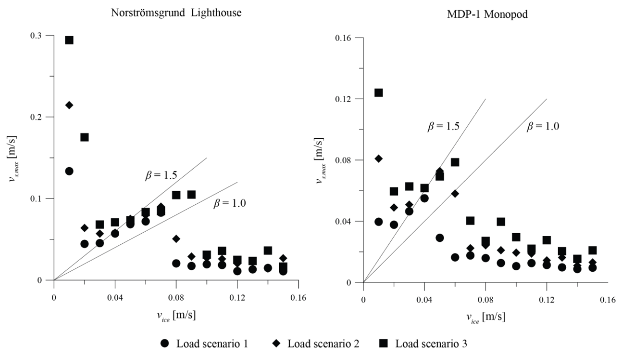
Figure 2. Left: Simulated dependence of maximum structural velocity on ice drift velocity for the Norströmsgrund lighthouse. Frequency lock-in is predicted to occur between 0.02 m/s and 0.09 m/s for the considered load scenarios. Right: Simulated dependence of maximum
