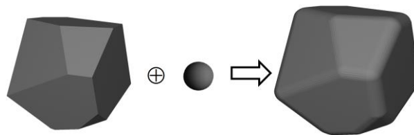
Figure 1. The dilated polyhedron generated by a basic polyhedron and a sphere.
