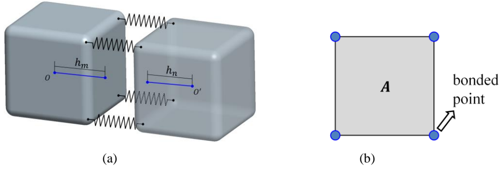
Figure 2. The common face of the adjacent elements: (a) Two adjacent elements; (b) The common face of the two adjacent elements, A is the area of the face.
