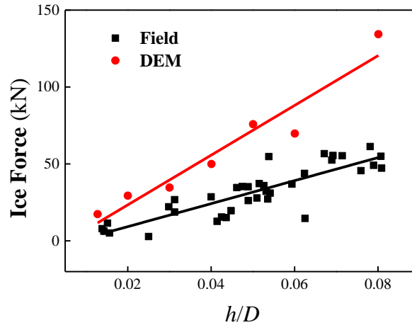
Figure 6. The ice load affected by the ratio between ice thickness and cone diameter. The ice loads in this figure are all maximum value. The field data of Bohai Sea is from Qu et al. (2006).
