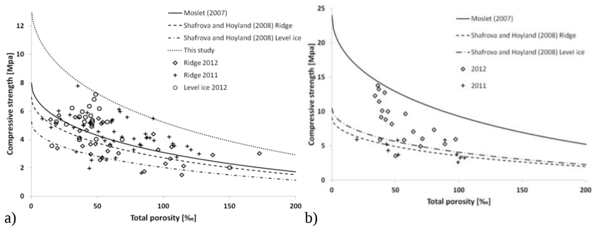
Figure 7. a) Horizontal and b) vertical compressive strength for all tested specimen at strain rate 10^{-3} \text{ s}^{-1} and temperature -10^\circ \text{ C} . The level ice samples are marked with a circle; all other samples are from consolidated layer. Trend lines expressing maximum compressive strength are added from earlier studies.
