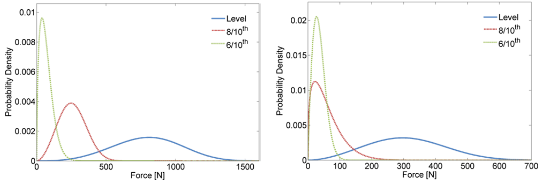
Figure 6. PDFs for 33 mm ice thickness, 22.5° orientation, a) full structure. b) design leg.
