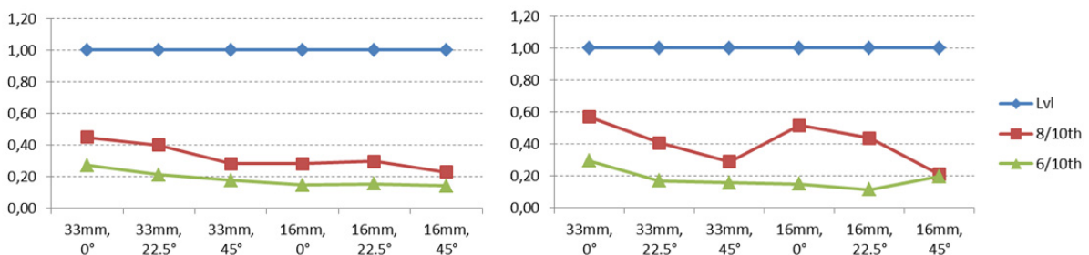
Figure 11. Ratios standard dev. for full scale velocity 1.0 m/s a) full structure. b) design leg.
