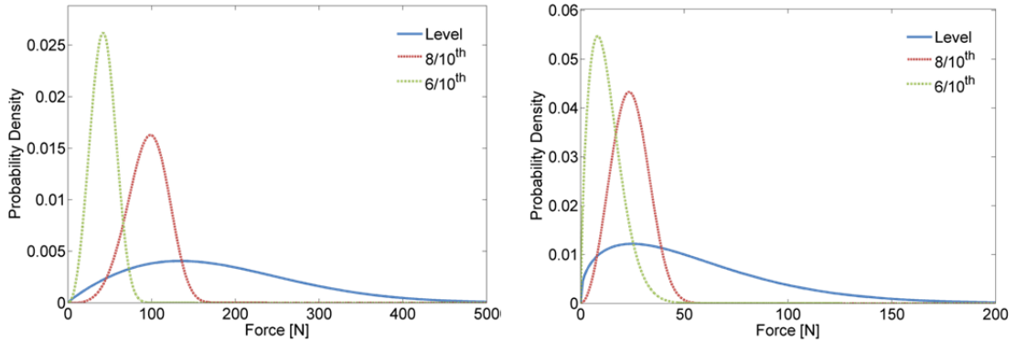
Figure 7. PDFs for 16 mm ice thickness, 45° orientation, a) full structure. b) design leg.
