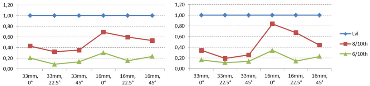
Figure 9. Mean load ratios for full scale velocity 1.0 m/s a) full structure. b) design leg
