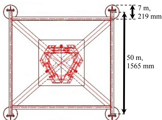
Figure 2. a) Dimensions of the jack-up in full scale and in model scale. b) The jack-up model at 22.5° orientation in level ice.
