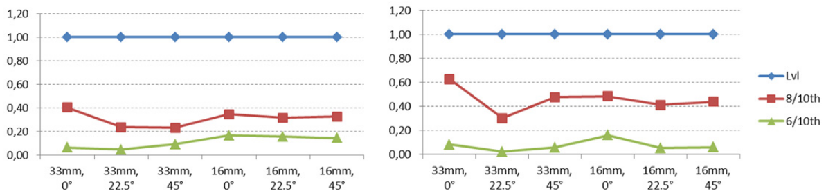
Figure 10. Ratios standard dev. for full scale velocity 0.5 m/s a) full structure. b) design leg.
