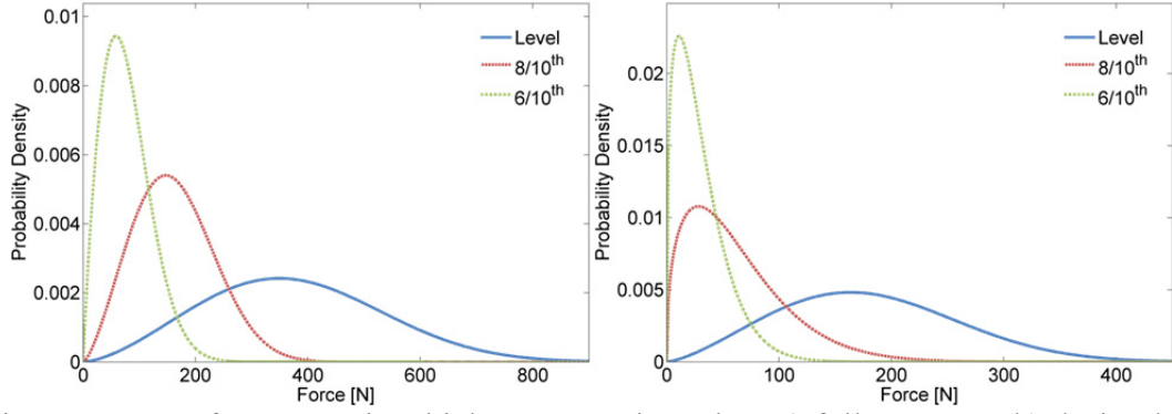
Figure 5. PDFs for 33 mm ice thickness, 0° orientation, a) full structure. b) design leg.
