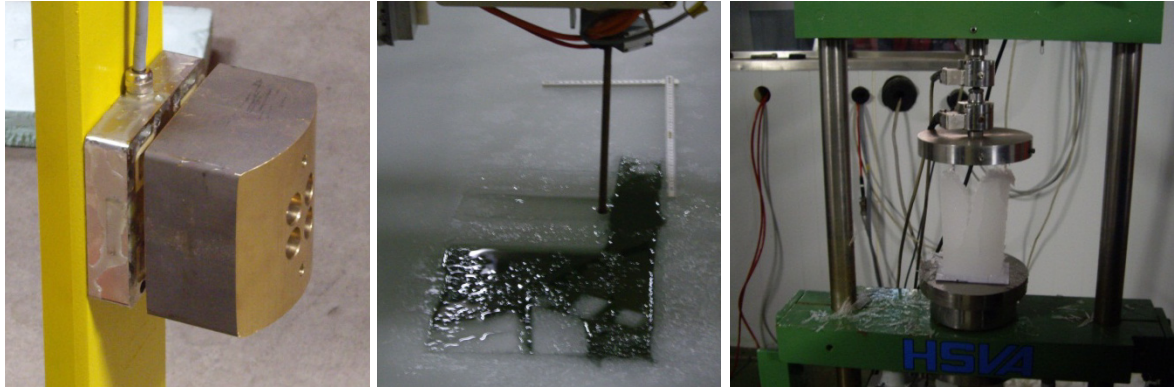
Figure 3. a) Tri-axial load cell for the jack-up legs attached to the jack-up model frame. b) In-situ bending test. c) Compression test.
