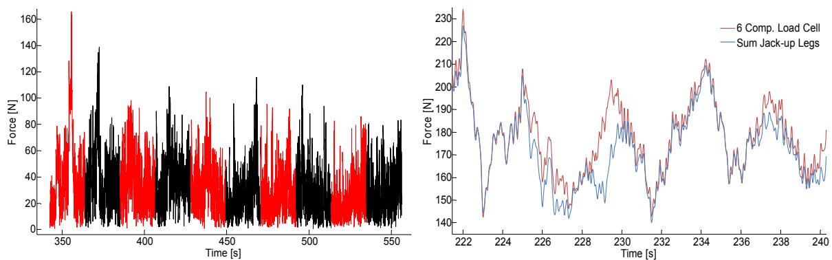
Figure 4. a) The resultant load on a front leg for test-run 11012 divided in 10 segments. b) Comparison: 6-component load cell versus the sum of the tri-axial load cells in the legs
