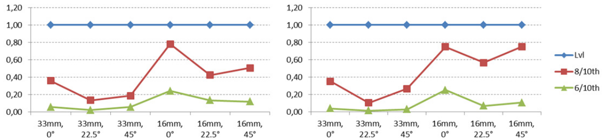
Figure 8. Mean load ratios for full scale velocity 0.5 m/s a) full structure. b) design leg
